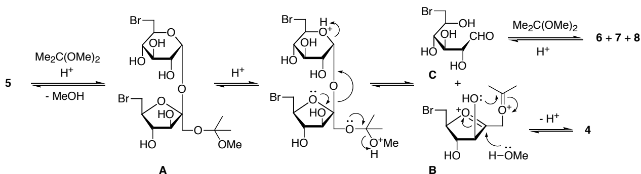
Scheme 2
