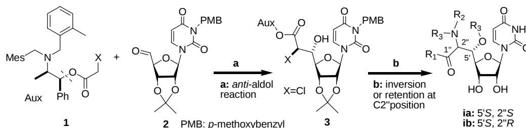
Scheme 2. Versatile strategy for the synthesis of uridine- \beta -hydroxylaminoesters.
