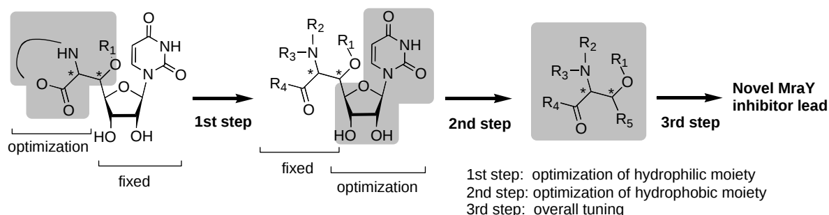
Scheme 1. Fragment-based design of novel MraY inhibitors.
