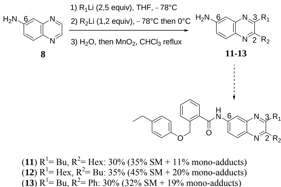
Scheme 3. Double organolithium addition to 6-aminoquinoxaline ( 8 )
