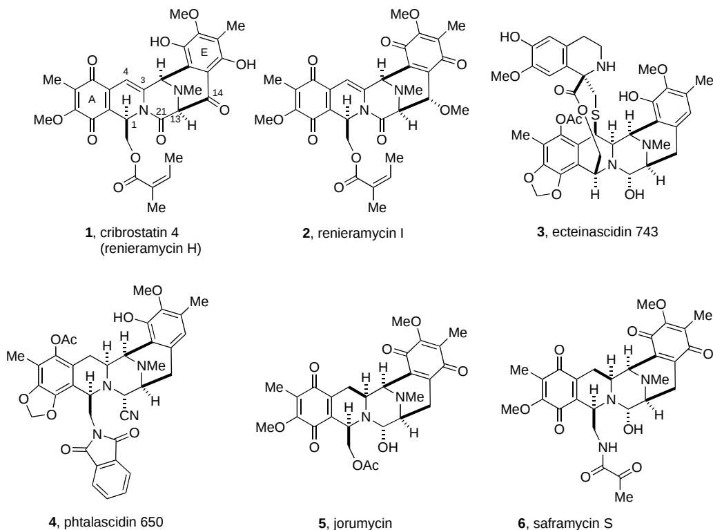
Figure 1. Tetrahydroisoquinoline alkaloids.
