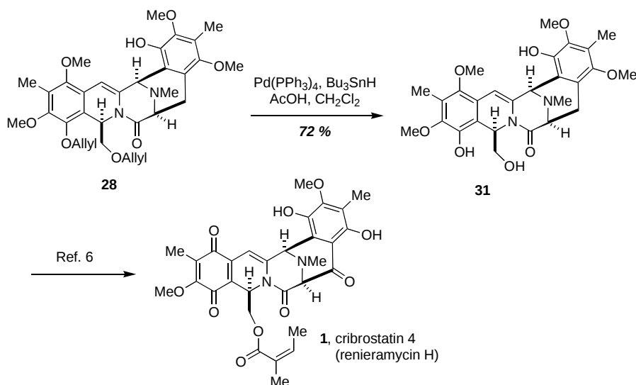
Scheme 9. Formal total synthesis of cribrostatin 4.
