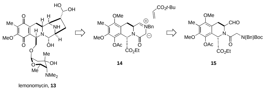
Scheme 3. Retrosynthesis of Lemonomycin.
