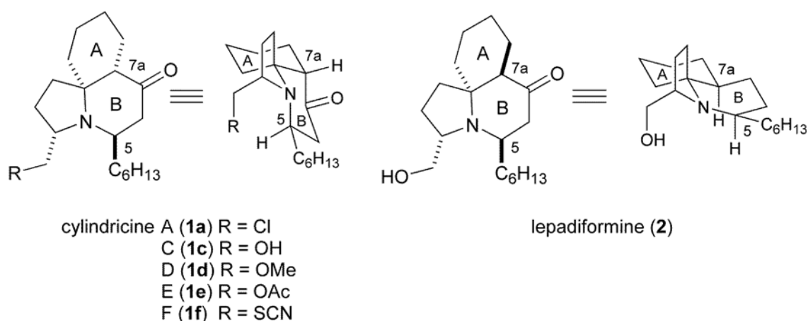
Figure 1. Tricyclic Marine Alkaloids, Cylindricines and Lepadiformine
