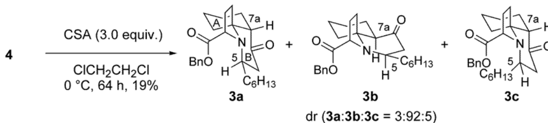
Scheme 7. Tandem Cyclization at 0 °C
