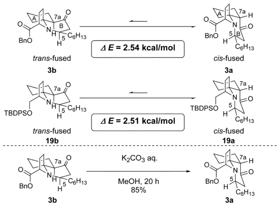
Scheme 6. Computational Analysis and Isomerization
