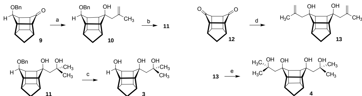
Scheme 2. Reagents and conditions: (a) \text{CH}_3(\text{CCH}_2)\text{CH}_2\text{MgCl} , THF, -78^\circ\text{C} , 97%. (b) \text{Hg}(\text{OAc})_2 , THF/ \text{H}_2\text{O} ; \text{NaBH}_4 , 3M NaOH, 89%. (c) \text{H}_2 (1 atm.), cat. Pd-C, EtOAc, 25^\circ\text{C} , 94%. (d) \text{CH}_3(\text{CCH}_2)\text{CH}_2\text{MgCl} , THF, reflux, 98%. (e) \text{Hg}(\text{OAc})_2 , THF/ \text{H}_2\text{O} ; \text{NaBH}_4 , 3M NaOH, 62%.
