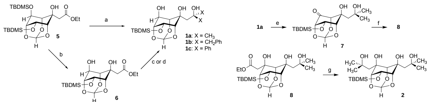
Scheme 1. Reagents and conditions: (a) \text{CH}_3\text{MgCl} , THF, 0 °C \rightarrow 25 °C, 85%. (b) 1 eq. TBAF, THF, 0 °C \rightarrow 25 °C, ref. 6. (c) \text{BnMgCl} , THF, rt, 61%. (d) \text{PhMgCl} , THF, reflux; isolation; \text{PhMgCl} , THF, reflux, 89% (two steps). (e) Dess-Martin periodinane, pyridine/ \text{CH}_2\text{Cl}_2 . (f) \text{EtOAc} , \text{LiHMDS} , THF, -78 °C, 81% (two steps); (g) \text{CH}_3\text{MgBr} , THF, 0 °C \rightarrow 25 °C, 69%.
