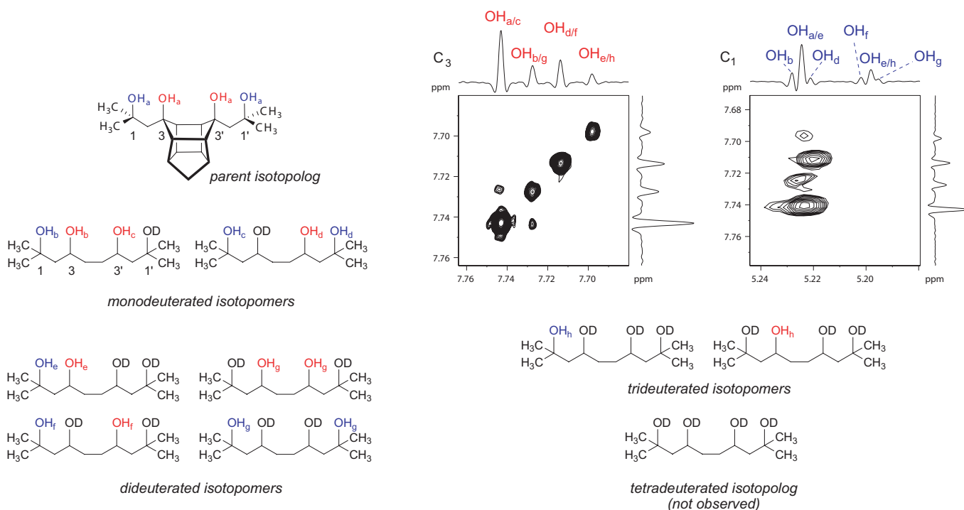
Figure 9. Isotopic perturbation of PCU tetrol 4 recorded at 40 °C in DMSO- d_6 . Left: C 1/1' and C 3/3' hydroxyl definitions for isotopically substituted species. Right: 400 MHz ^1\text{H} 2D COSYLR spectra for partially deuterated tetrol 4 , with hydroxyl resonance assignments. Left spectrum: region corresponding to the C 3 -OH hydroxyl group. The single off-diagonal correlation is evidence for C 3 -OH a /OH b scalar coupling. Right spectrum: region showing C 3 -OH/C 1 -OH coupling partners.
