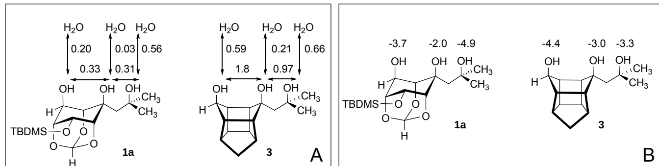
Figure 5. (A) A comparison of magnetization exchange rate constants (s -1 ) obtained from 2D EXSY spectra for triols 1a and 3 in DMSO- d_6 at 80 °C. (B) A comparison of OH chemical shift temperature coefficients (ppb K -1 ) measured in DMSO- d_6 .
