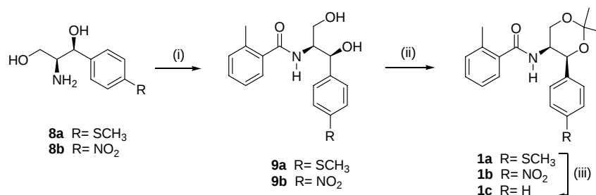
Scheme 2 Reagents and conditions: (i) o -toluoyl chloride, 0.5M KOH, \text{CH}_2\text{Cl}_2 , 0\text{ }^{\circ}\text{C} ; (ii) (\text{CH}_3\text{O})_2\text{C}(\text{CH}_3)_2 , acetone, \text{H}_2\text{SO}_4 , rt; (iii) Raney nickel, EtOH, rt.
