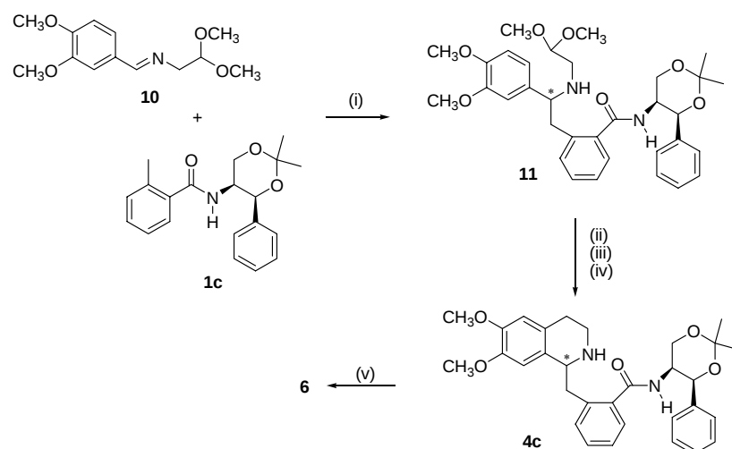
Scheme 3 Reagents and conditions : (i) n -BuLi (2.2 equiv), THF, Ar, -72\text{ }^{\circ}\text{C} ; (ii) column chromatography separation; (iii) 6M HCl, rt; (iv) \text{H}_2 , Pd/C, HCl/MeOH; (v) toluene, reflux.
