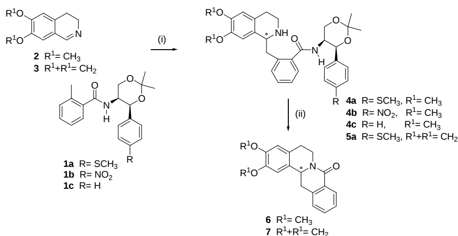
Scheme 1 Reagents and conditions: (i) n -BuLi (2.2 equiv), THF, Ar, -72\text{ }^{\circ}\text{C} ; (ii) toluene, reflux.
