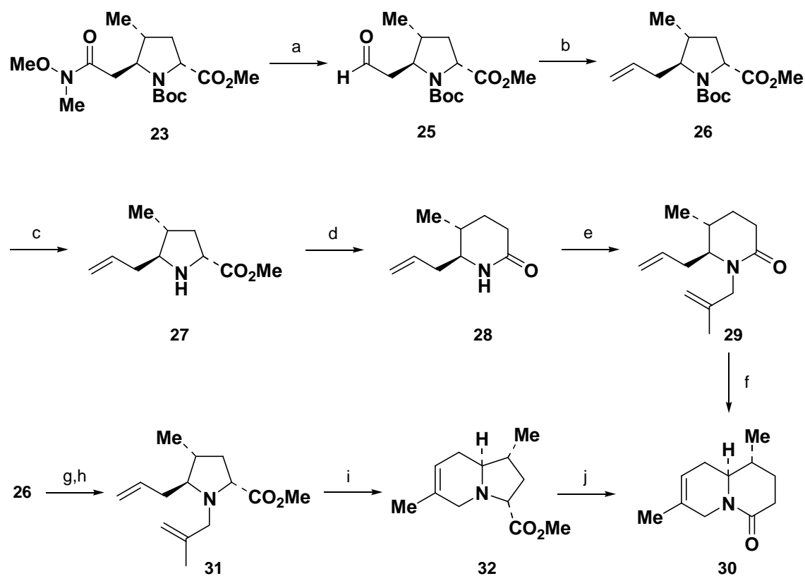
Scheme 6. Reagents and conditions: (a) DIBAL, THF, -78^{\circ}\text{C} ; (b) NaHMDS, \text{Ph}_3\text{PCH}_3^+\text{Br}^- , THF, -78^{\circ}\text{C} to rt (95% from 23 ); (c) TFA, \text{CH}_2\text{Cl}_2 , 0^{\circ}\text{C} to rt; (d) \text{SmI}_2 , THF, HMPA, MeOH, 0^{\circ}\text{C} to rt (90% from 26 ); (e) 3-bromo-2-methylpropene, NaH, DMF, 0^{\circ}\text{C} to rt (87%); (f) 2 mol% Grubbs' 2nd cat., benzene, 60^{\circ}\text{C} (96%); (g) TFA, \text{CH}_2\text{Cl}_2 , 0^{\circ}\text{C} to rt; (h) 3-bromo-2-methylpropene, NaH, DMF, 0^{\circ}\text{C} to rt (88% from 26 ); (i) 2 mol% Grubbs' 2nd cat., benzene, 60^{\circ}\text{C} (70%); (j) \text{SmI}_2 , THF, HMPA, MeOH, 0^{\circ}\text{C} to rt (82%)
