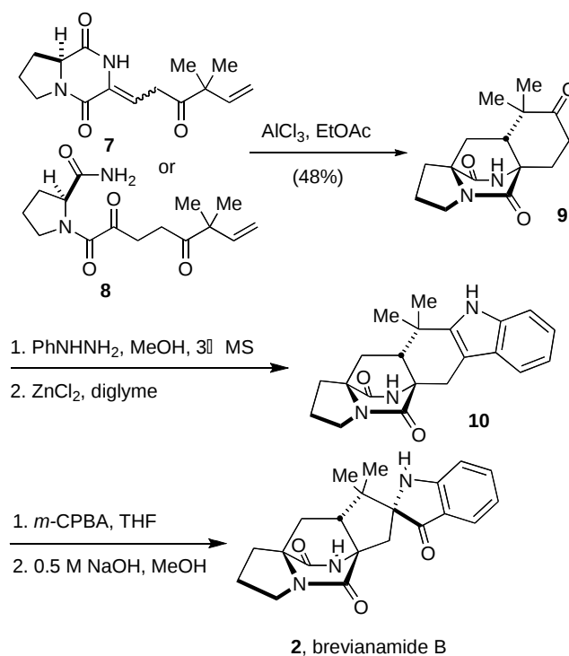
Scheme 1. The concise synthesis of brevianamide B ( 2 ).
