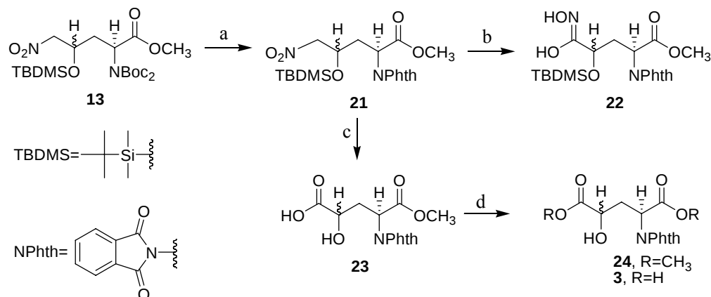
Scheme 4. Reagents and Conditions: (a) TFA/CH 2 Cl 2 then TEA/THF/ N -carbethoxyphthalimide/16 h/reflux 2 h, 68%; (b) NaNO 2 (3 eq)/AcOH (10 eq)/DMSO/rt/16 h, 16%; (c) NaNO 2 (3 eq)/AcOH (10 eq)/DMSO/40°C/17 h, 51%; (d) TMSCl/MeOH/rt/20 h, 90%.
