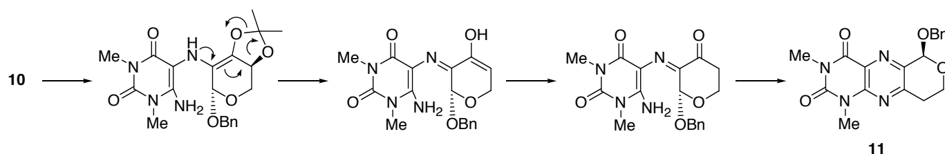
Scheme 3
