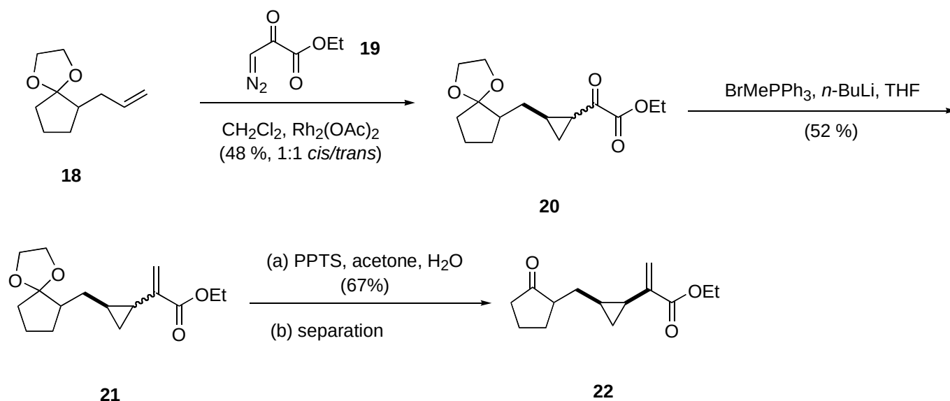
Scheme 5. Synthesis of Vinylcyclopropane ( 22 )
