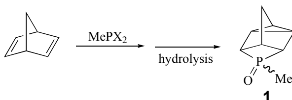
Scheme 2. Formation of 4-methylphosphatetracyclo[3.3.0,0 2,8 ,0 3,8 ]octane 4-oxides
