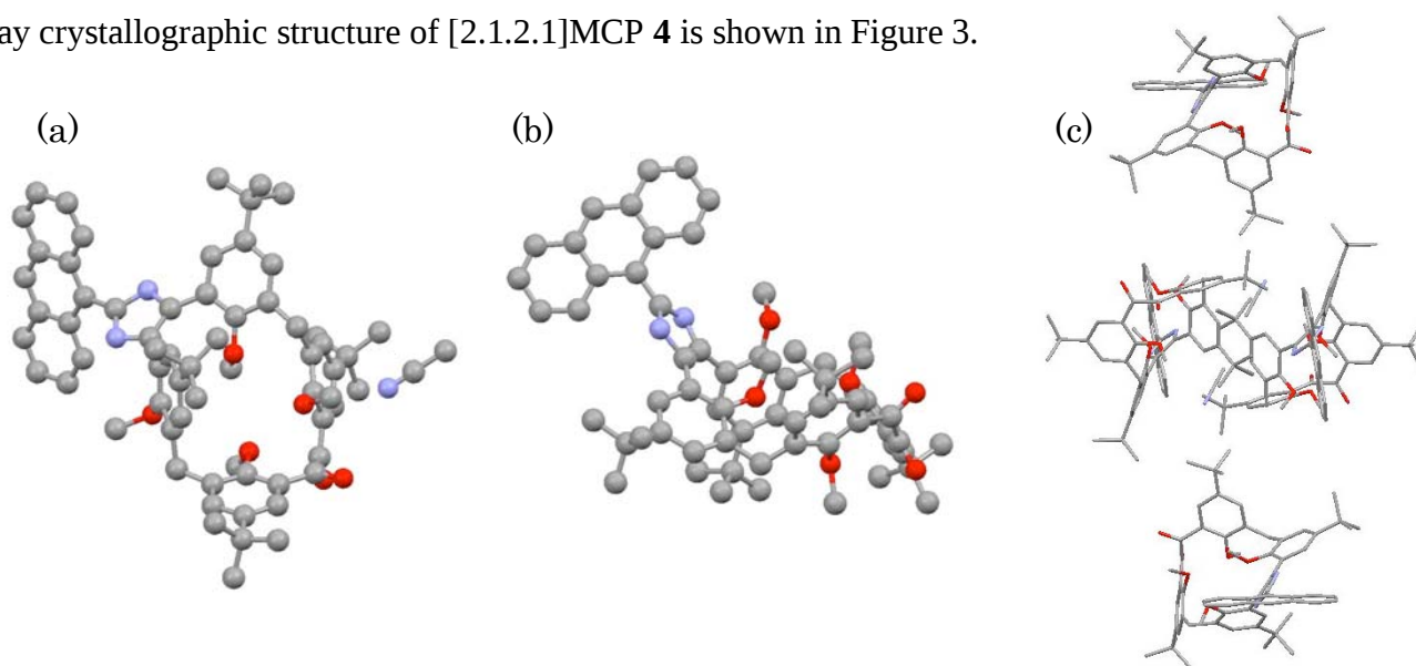
Figure 3. X-Ray crystallographic structure of [2.1.2.1]MCP 4 :
