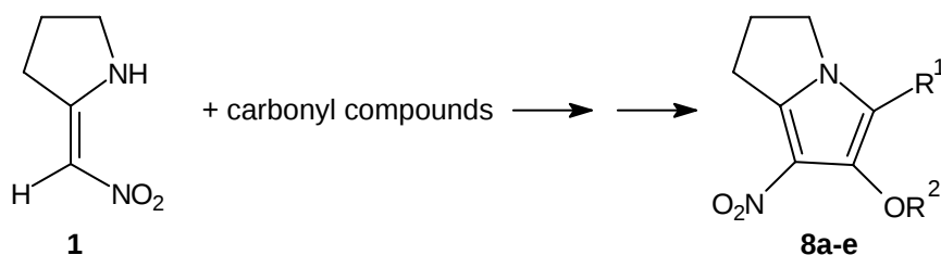
Scheme 1. Formation of substituted pyrrolizines.
