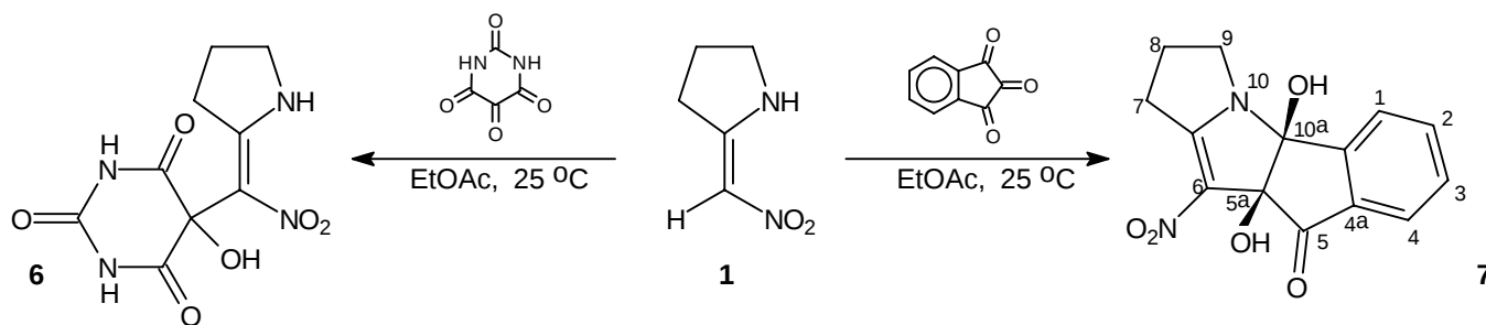
Scheme 5. Reaction of 1 with alloxan and ninhydrin.
