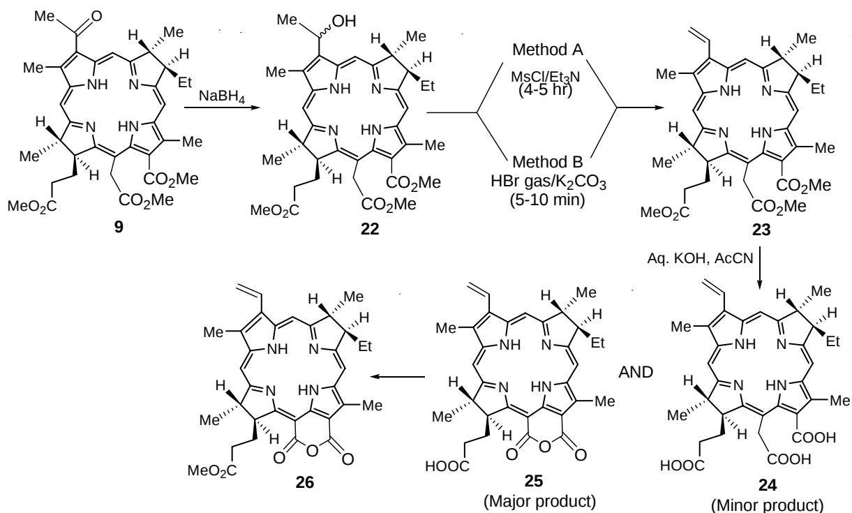
Scheme 7: Bacteriochlorins with 3-vinyl substituents
