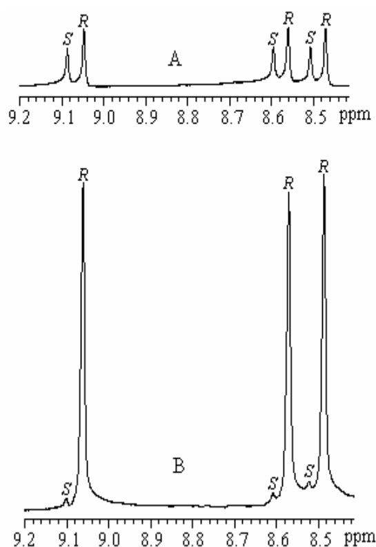
Figure 1: Partial NMR spectra (only the meso region is shown) of methyl 13 2 -hydroxy bacteriopheophorbide-a. A: The diastereomeric mixture obtained by reacting 7 with (+)-( 1S )-(10-camphorsulfonyl) oxaziridine[(+) 12b ]. The ratio of R - and S -isomers was 60 to 40. B: The diastereomeric mixture obtained by reacting 7 with (-)-( 1R )-(10-camphorsulfonyl) oxaziridine [(-) 12a ]. The ratio of R - and S -isomers was 95 to 5.
