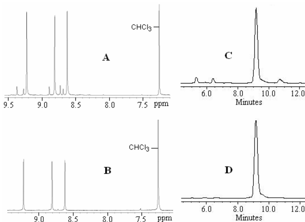
Figure 2: A and B : Partial NMR spectra (only the meso -region is shown) of crude reaction mixture obtained by reacting 17 with L-aspartyl-di-tert-butyl ester in the presence of EDCI and DMAP and the pure imide analog 21 and the C and D are the HPLC profiles (C-18 column, eluting solvent 90% methanol in water) of the crude and pure isomide 21 respectively (for details see the text).
