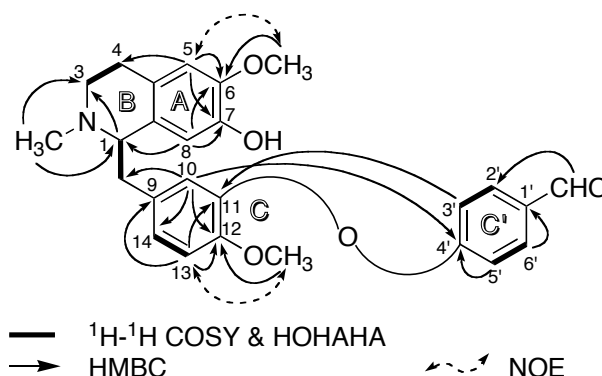
Figure 1. Selected 2D NMR correlations for peccassipine A ( 1 )
