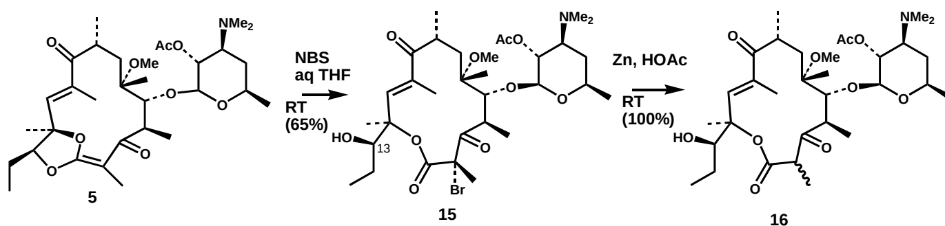
Scheme 4
