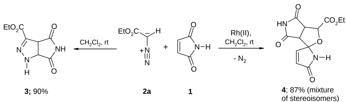
Scheme 3. Reactions of diazoacetate ( 2a ) with maleimide ( 1 ) in the absence and presence of \text{Rh}_2(\text{OAc})_4
