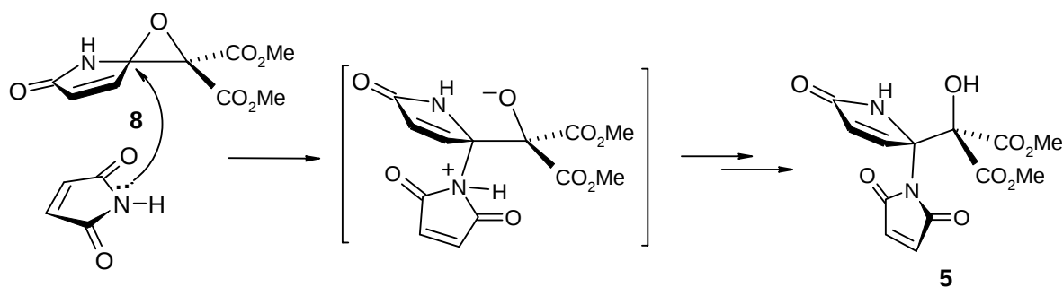
Scheme 7. Nucleophilic ring-opening of the oxirane ( 8 )
