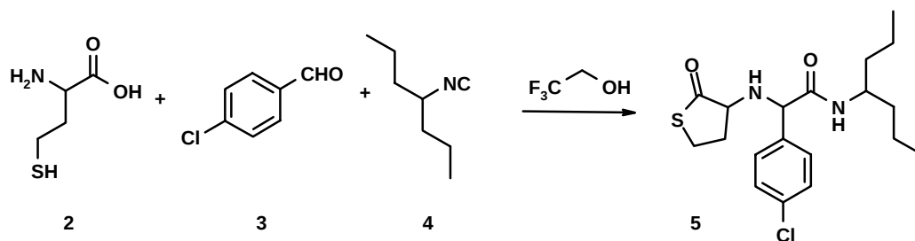
Scheme 2. The reaction of homocysteine 2 , 4-chlorobenzaldehyde 3 and 4-isocyanoheptane 4 in TFE yields 5 .
