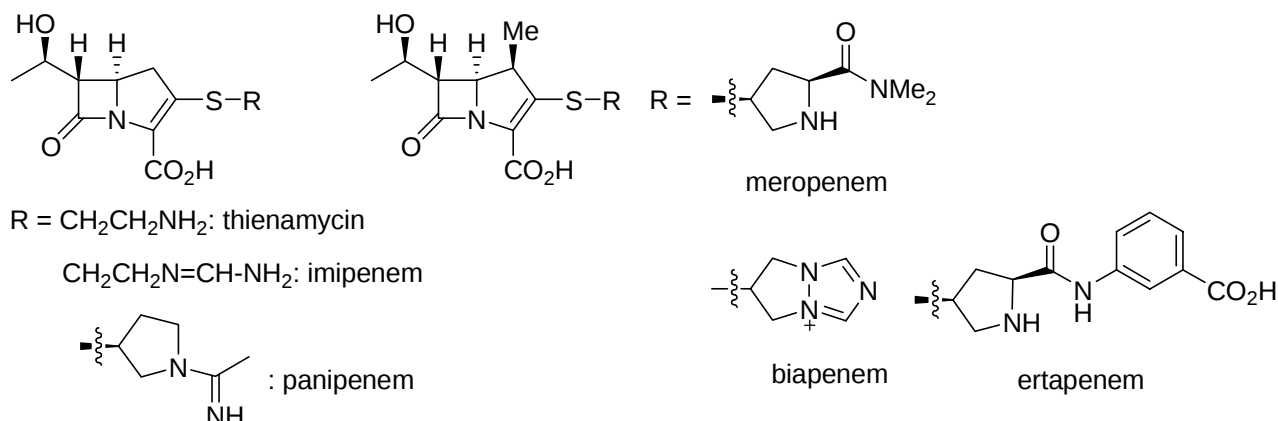
Scheme 1. Carbapenems
