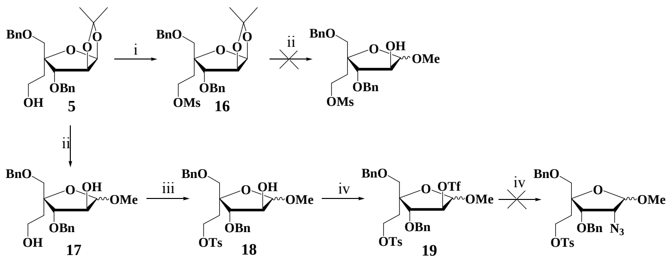
Scheme 2. Reagents and conditions: (i) MsCl, pyridine, 0 °C, 1 h; (ii) MeOH, H 2 SO 4 , reflux, 0.5 h; (iii) p -toluenesulfonyl chloride, pyridine, 0 °C to rt, overnight; (iv) Tf 2 O, pyridine, CH 2 Cl 2 , 0 °C, rt, 0.3 h; then NaN 3 , DMF, 40 °C, 48 h.
