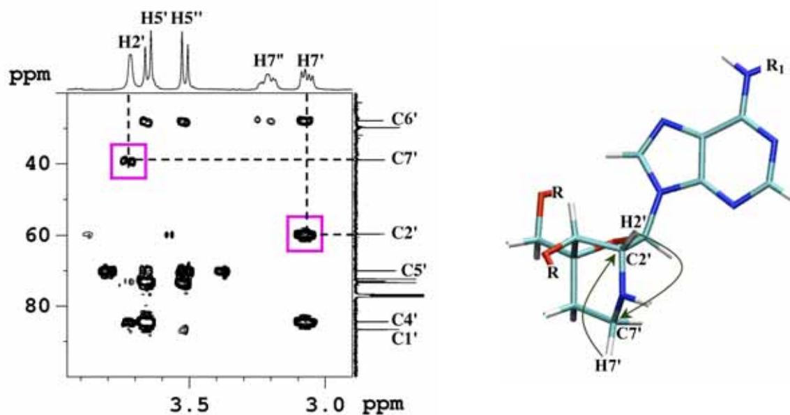
Figure 7. Expansion of HMBC spectrum of 13 ( R = Bn , R 1 = Bz ) showing important ^3J_{\text{HC}} correlations confirming the ring closure between 2'C and 2'N, forming the 6-membered piperidino ring. H2' shows the ^3J_{\text{HC}} correlation to C7' and H7' shows the ^3J_{\text{HC}} correlation to C2'. The presence of the correlation of only H7' to C2' indicates that the dihedral angle between H7' and C2', \phi[\text{H7'-C7'-N-C2'}] , is closer to 180°.
