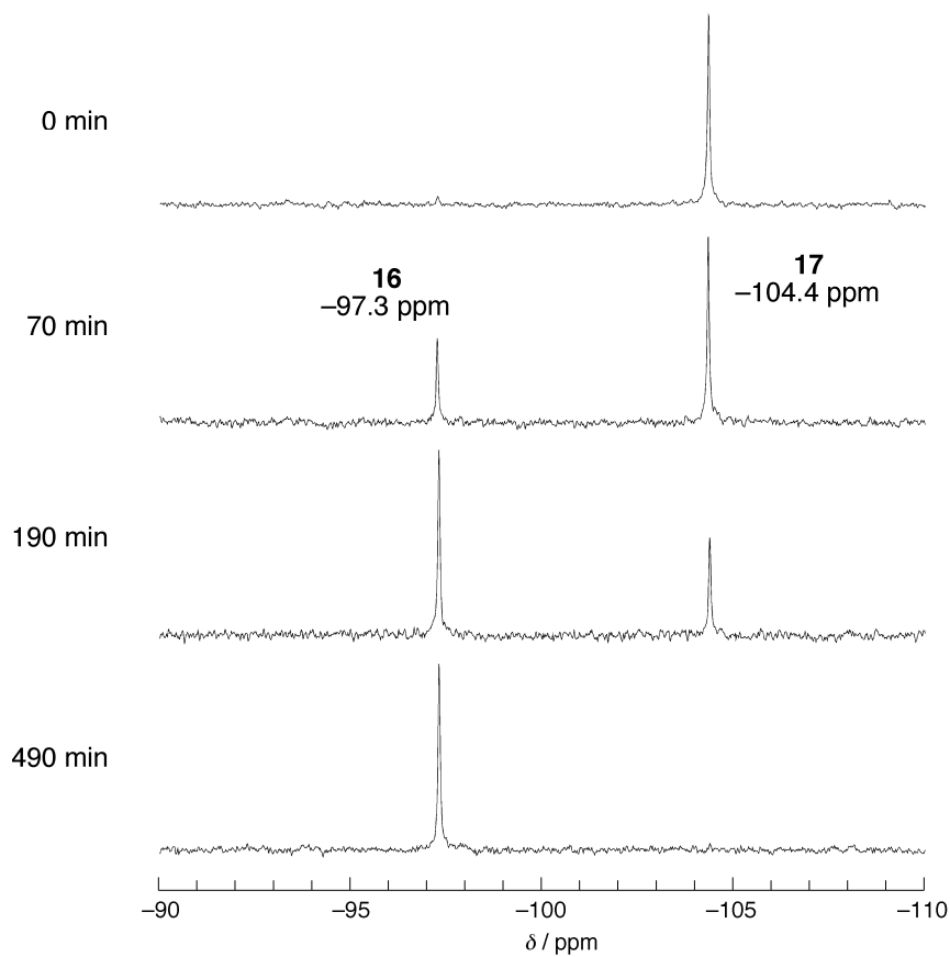
Figure 5. Time course of the ^{31}\text{P} NMR for the conversion of 17 to 16 at 60 °C in THF.
