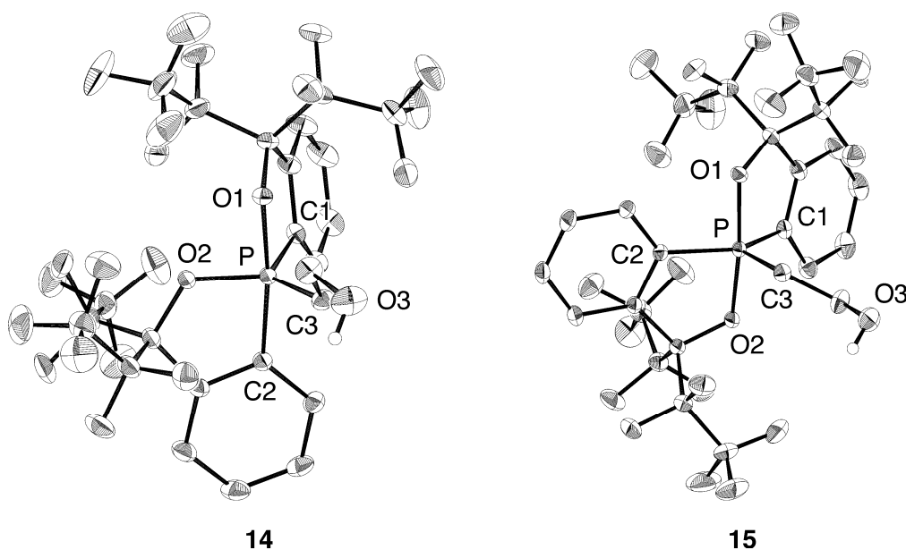
Figure 4. The ORTEP drawings of β -hydroxyethylphosphoranes ( 14 and 15 ) showing the thermal ellipsoids at the 30% probability level. The hydrogen atoms, except for the hydroxyl proton, are omitted for clarity.
