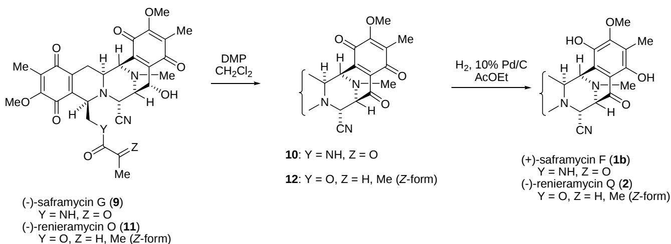
Scheme 5
