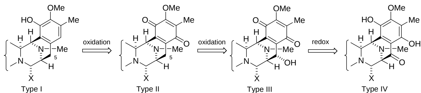
Scheme 1
