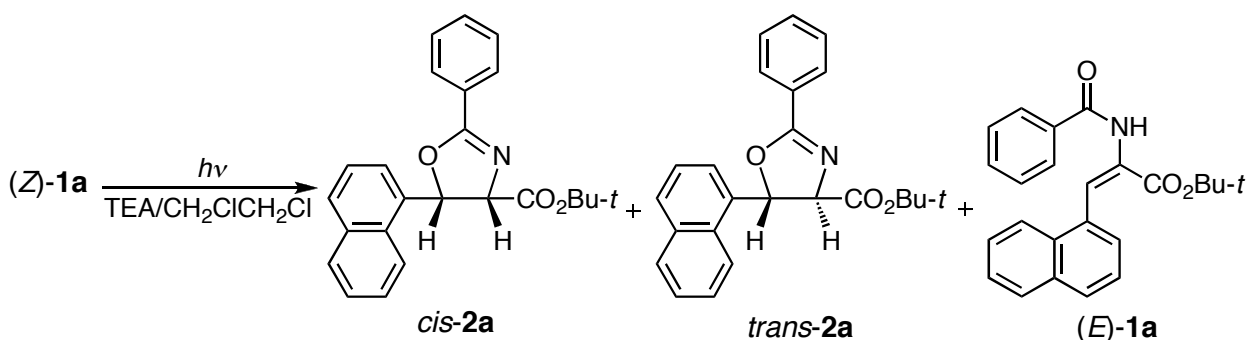
Scheme 1
