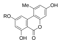
1: R = H: alternariol 2: R = Me: alternariol 9-methyl ether
