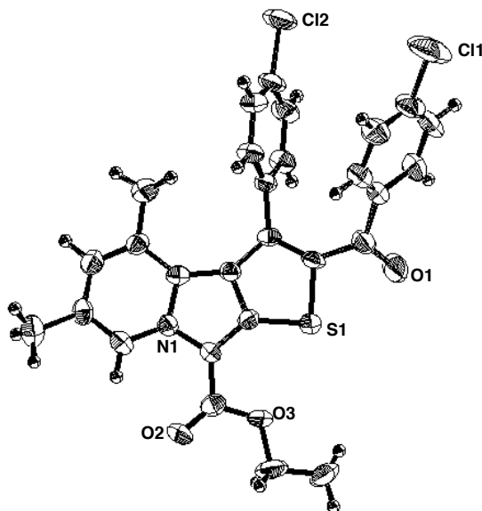
Figure 3. ORTEP drawing of compound 7e
