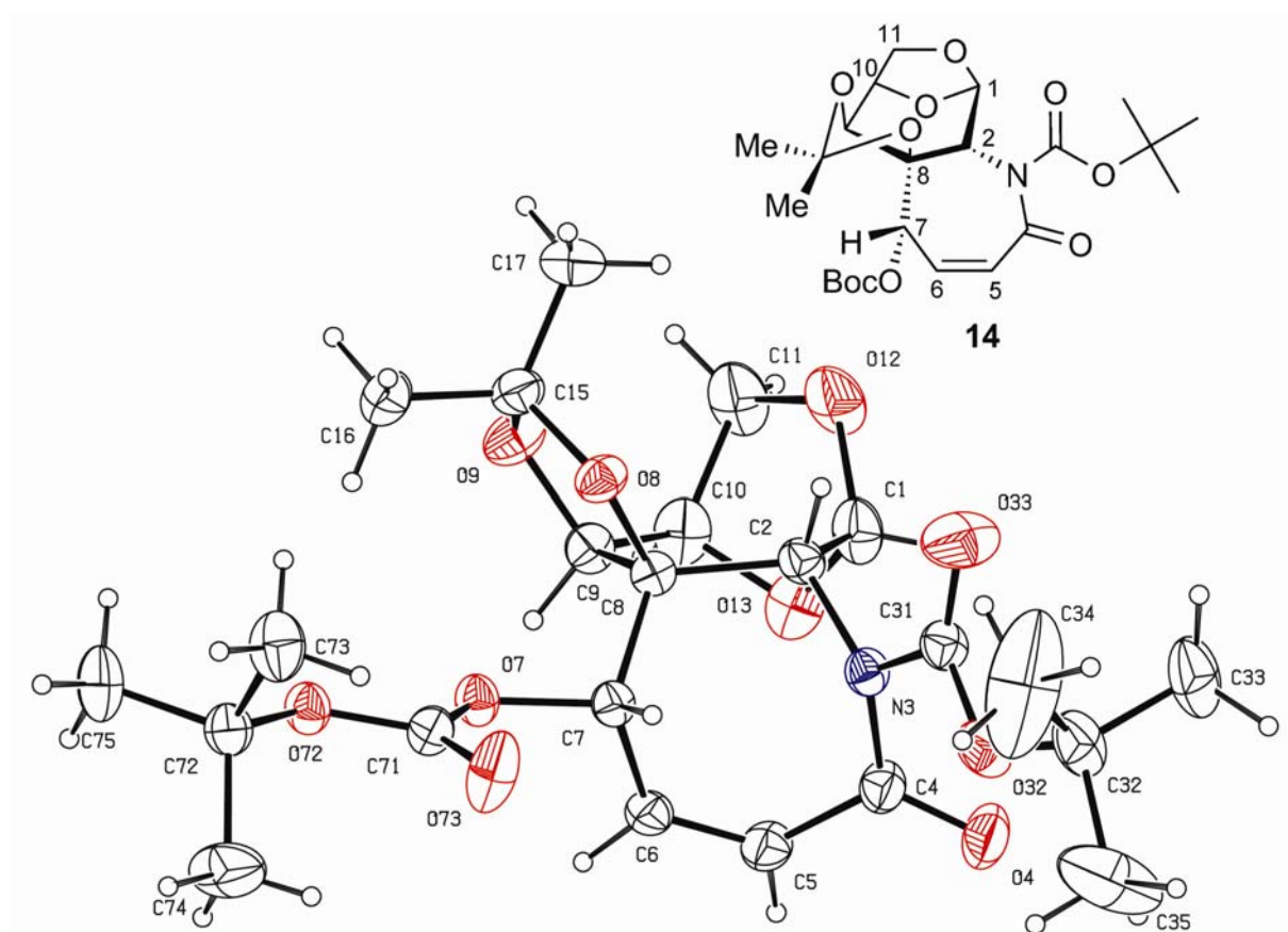
Figure 1. X-Ray structure of \alpha,\beta -unsaturated lactam 14 .
