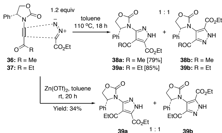
Scheme 7. [3 + 2] Cycloadditions of Push-Pull-Ynamides
