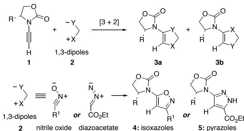
Scheme 2. Cycloadditions with Nitrile Oxide and Ethyl \alpha -Diazooacetate
