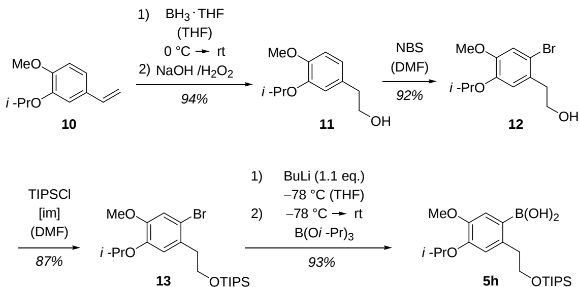
Scheme 3. Preparation of boronic acid 5h from styrene 10 .
