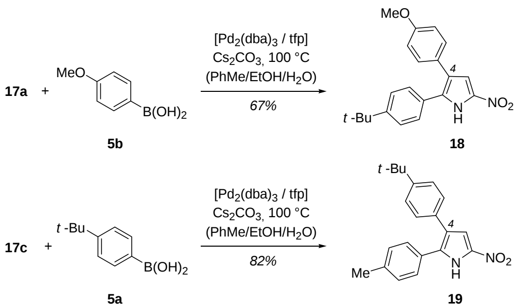
Scheme 5. Synthesis of 4,5-diarylpyrroles 18 and 19 by successive Suzuki cross-coupling reactions.
