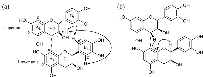
Figure 3. Important 2D-NMR correlations observed for 7 , indicating the location (C-4 U →C-8 L ) of the flavan linkage, (a) ROE (H↔H) and (b) HMBC (H→C).
