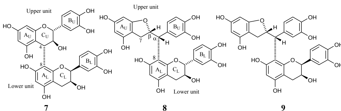
Figure 2. Structures of compounds 7–9 newly isolated from gambir.
