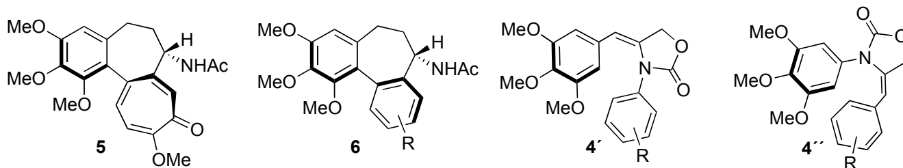
Scheme 2. Bioactive molecules with a trimethoxyaryl unit adopting a twisted conformation
