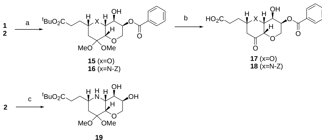
Scheme 5. Double bond functionalisation, reagents and conditions : (a) benzoylchloride, DMAP Et 3 N, CH 2 Cl 2 , yield: 89 % ( 15 ), 49 % ( 16 ); (b) TFA, CH 2 Cl 2 , yield: 96 % ( 17 ), 83 % ( 18 ); (c) Pd/C, H 2 , MeOH, yield: 98 % ( 19 ).
