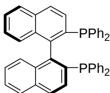
(S)-BINAP
