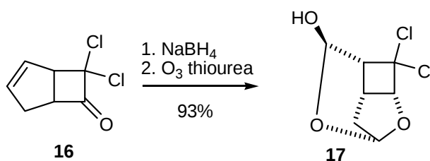
Scheme 3. Synthesis of crystalline compound 17
