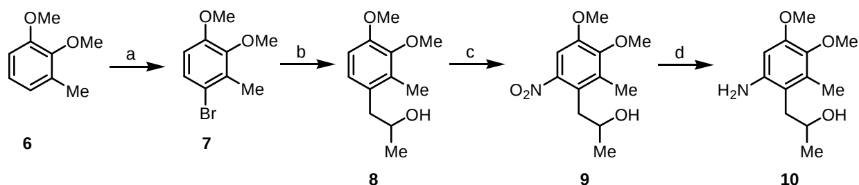
Scheme 2. Synthesis of the arylamine 10 . Reagents and conditions. (a) NBS, MeCN, rt, 27 h, 96%; (b) BuLi, THF, -78^{\circ}\text{C} , 15 min, ( \pm )-propene oxide, -78^{\circ}\text{C} to rt, 18 h, 89%; (c) 100% \text{HNO}_3 , HOAc, \text{CH}_2\text{Cl}_2 , 0^{\circ}\text{C} to rt, 2 h, 47%; (d) \text{H}_2 , 10% Pd/C, MeOH, rt, 1.5 h, 93%.
