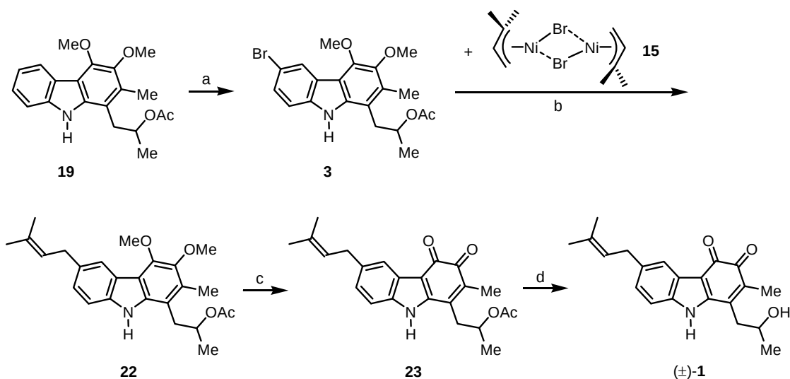
Scheme 8. Synthesis of (±)-carquinostatin ((±)- 1 ). Reagents and Conditions : (a) NBS, \text{CCl}_4 , 77 °C, 30 min, 93%; (b) DMF, 65 °C, 15 h, 81%; (c) CAN, MeCN/ \text{H}_2\text{O} , 0 °C, 30 min, 62%; (d) \text{LiAlH}_4 , THF, rt, 22.5 h, 61%.
