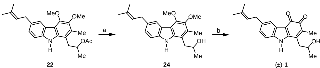
Scheme 9. Synthesis of (±)-carquinostatin ((±)- 1 ). Reagents and Conditions : (a) KOH, MeOH/ \text{H}_2\text{O} , rt, 3 h, 95%; (b) CAN, MeCN/ \text{H}_2\text{O} , 0 °C, 30 min, 64%.
