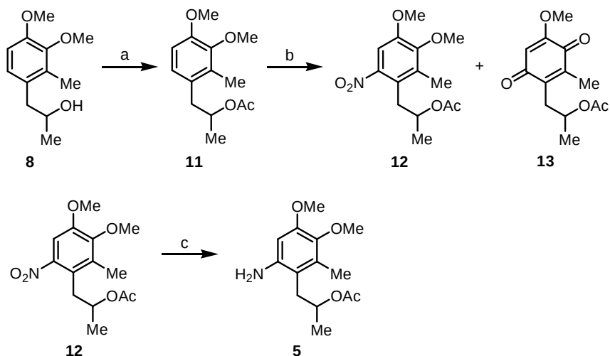
Scheme 3. Synthesis of the arylamine 5 . Reagents and conditions: (a) \text{Ac}_2\text{O} , \text{Et}_3\text{N} , DMAP, \text{CH}_2\text{Cl}_2 , rt, 1 h, 97%; (b) 100% \text{HNO}_3 , \text{Ac}_2\text{O} , HOAc, \text{CH}_2\text{Cl}_2 , 0^{\circ}\text{C} , 1.5 h, 89% 12 , 6% 13 ; (c) \text{H}_2 , 10% Pd/C, MeOH, rt, 5 h, 94%.
