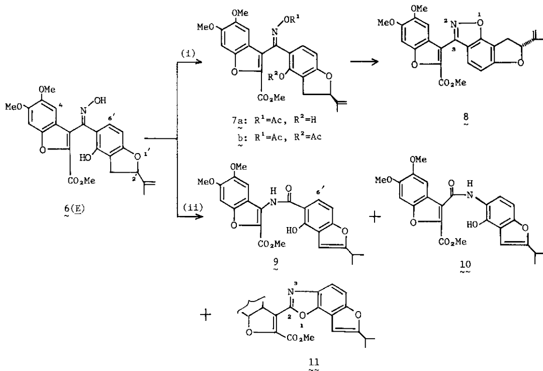
Chart 2. Reagents : (i) Ac 2 O/pyridine; (ii) PPA
