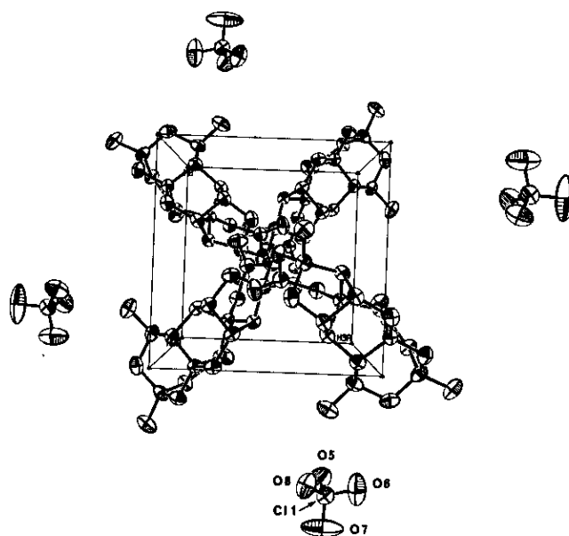
Figure 2. ORTEP Plot of 4·Perchlorate Unit Cell
