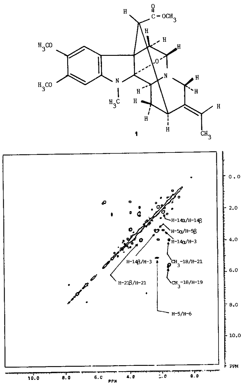
Fig. 1: COSY 45° spectrum of (+)-alstipicalamine (1)
