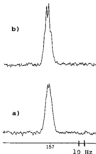
Fig. 2 LSPD spectra of 1 a) Reference spectrum, irradiation at \delta 12.17 and 12.73 ppm (triple irradiation). b) Irradiation at \delta 2.63 and 2.81 ppm ( \text{H}_2 -4), (triple irradiation).
