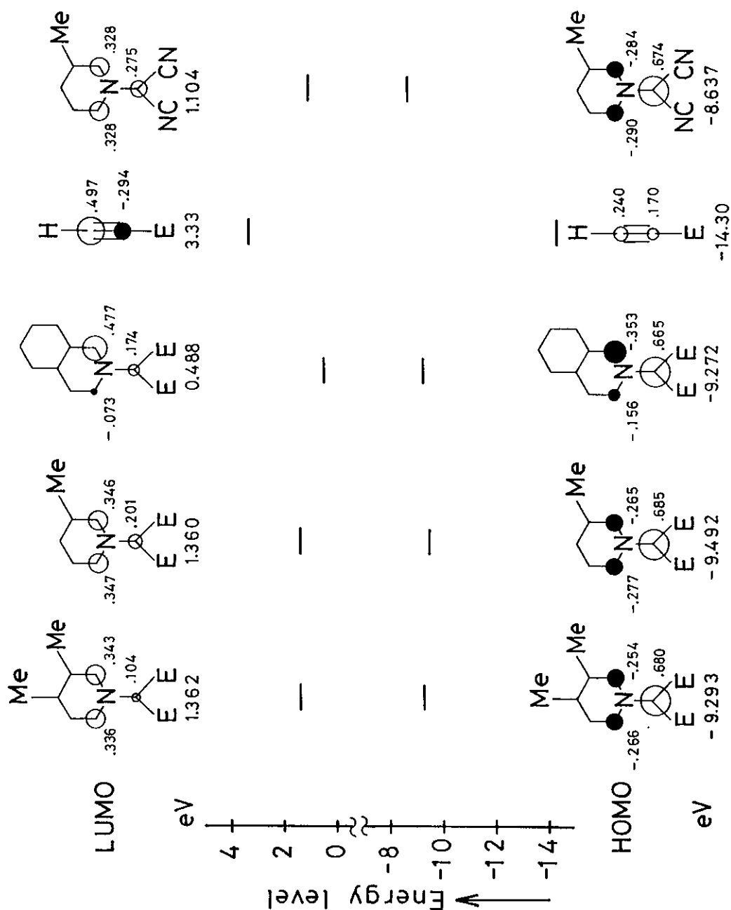
Fig. 1. Frontier molecular orbital interaction in 1,3-dipolar cycloaddition of 1a , b , c and 2-methylpyridinium dicyanomethylide with 2.
