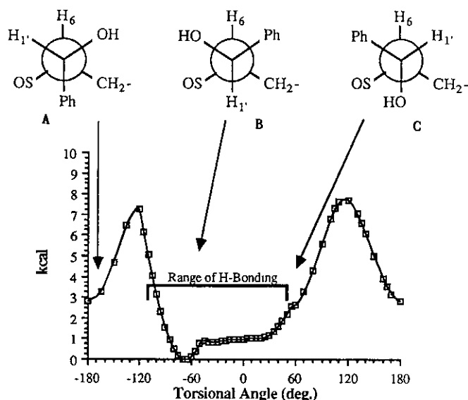
Potential energy of \mathbf{2} as a function of the H(6)-C(6)-C(1)-Ph torsion angle
