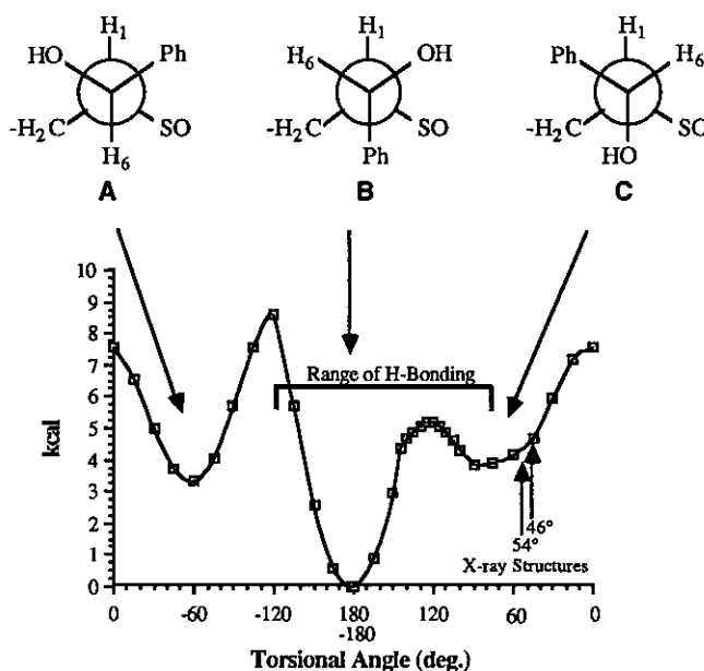
Calculated potential energy of \mathbf{1} as a function of the H(1)-C(1)-C(6)-Ph torsional angle
