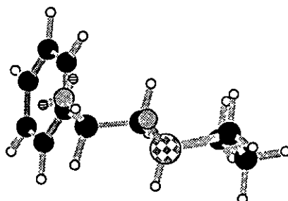
Optimal conformation of \tilde{2} (calculated)
