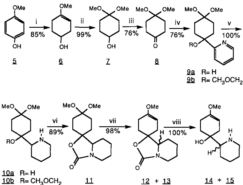
SCHEME 1. Reagents (see the Experimental for details) i: \text{LiNH}_2 , then EtOH; 5 ii: \text{CH}(\text{OCH}_3)_3 , p\text{-TsOH}/\text{C}_6\text{H}_6\text{-MeOH} ; ii: \text{CrO}_3(\text{C}_5\text{H}_5\text{N})_2/\text{CH}_2\text{Cl}_2 6 (yield after chromatographic purification); iv: 2-pyridyllithium / THF (yield of recrystallized product); v: \text{H}_2 , 5% Ru-C / THF-H 2 O; vi: \text{COCl}_2 , Et 3 N (2 eq) / \text{CH}_2\text{Cl}_2 ; vii: Et 3 NHCl (10-15% by weight), 180°C; viii: KOH/MeOH-H 2 O, 110-120°C (sealed tube).
