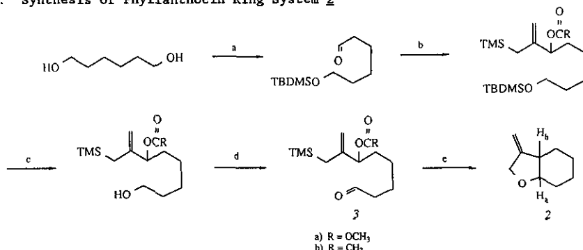
Scheme 1. Synthesis of Phyllanthocin Ring System 2
