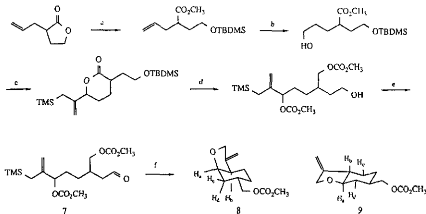
Scheme 2. Cyclization to Substituted Phyllanthocin Ring System
