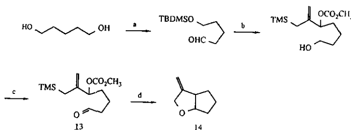
Scheme 3. Synthesis of 4-Methylene-2-oxabicyclo[3.3.0]octane ( 14 )
