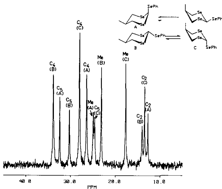
Figure 3. ^{13}\text{C} Nmr spectrum of a mixture of cis and trans -5-methyl-2-phenylseleno-1,3-diselenane 10 in \text{CFCl}_3:\text{CD}_2\text{Cl}_2 (85:15) at 147°K.
