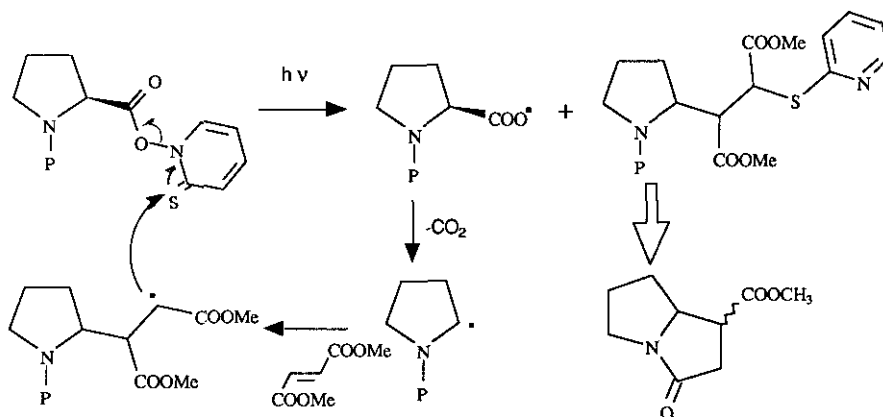
Scheme I
