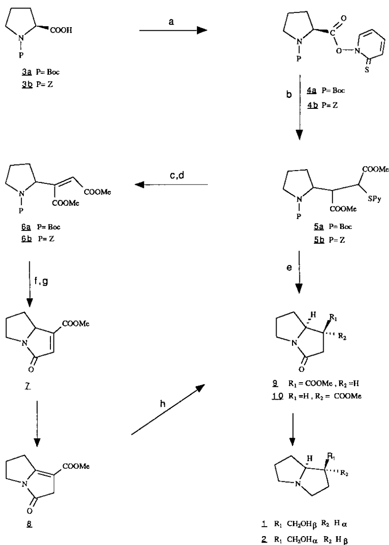
Scheme II
