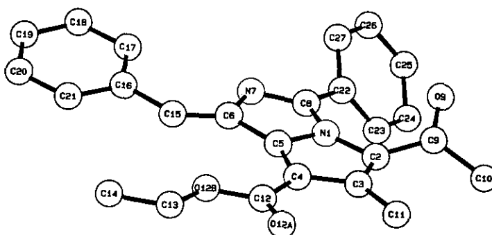
Figure 1: The solid state conformation of 6h . Hydrogen atoms have been omitted for clarity.
