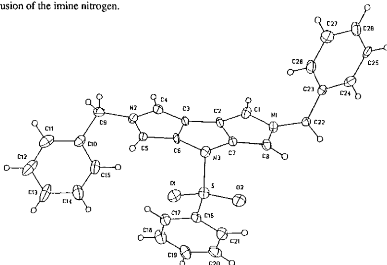
Figure 1: Molecular drawing of 23 generated by SHELXTL PLUS.
