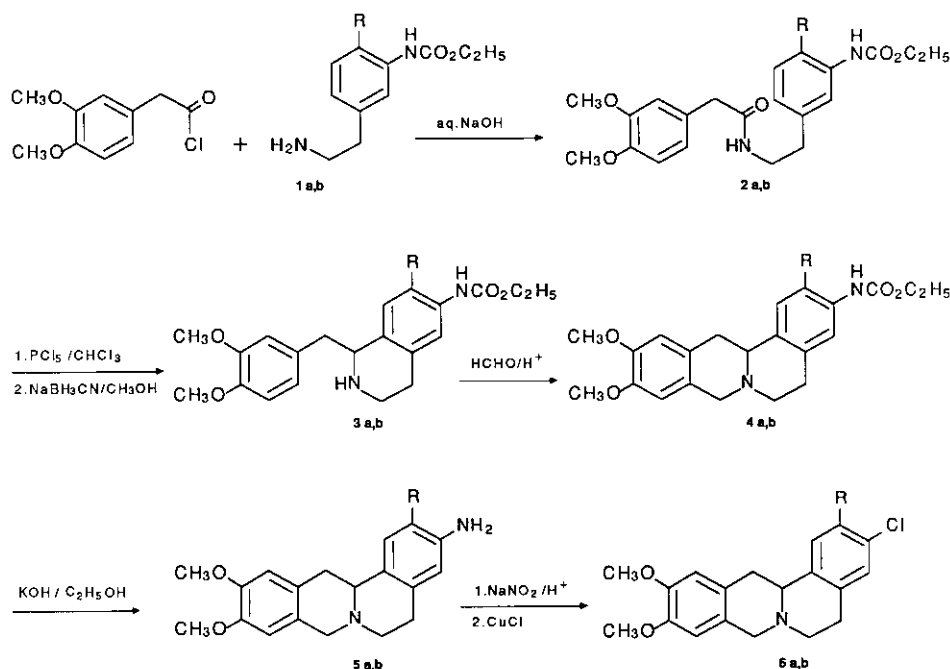
Scheme 1. Chlorination of berbine in the ring A ( a : R=H, b : R=Cl)
