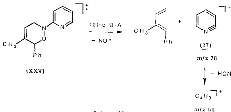
Scheme 14a
