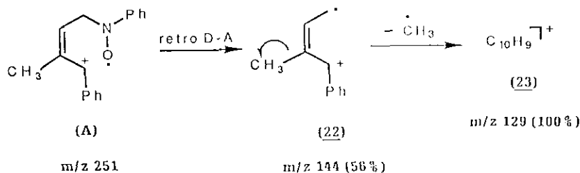
Scheme 11a
