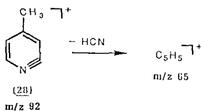
Scheme 14b
