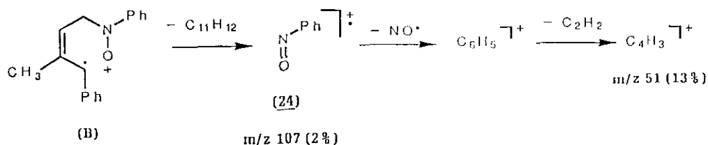
Scheme 11b
